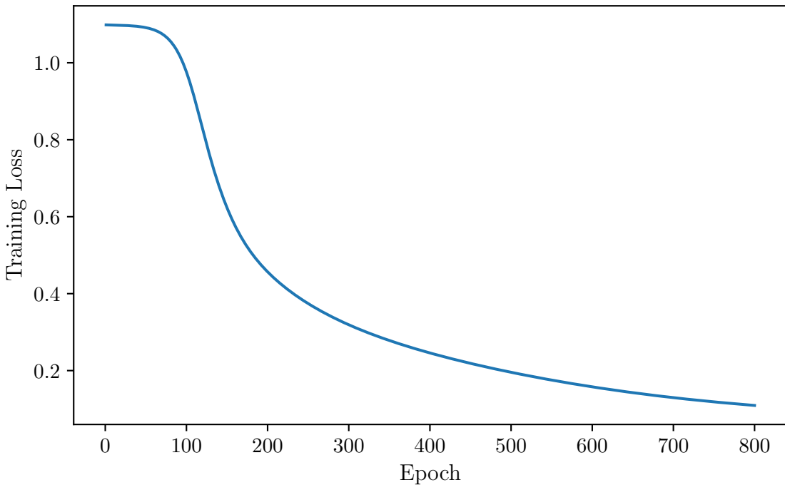
Training Loss over Epochs
